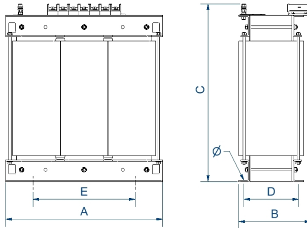
Dimensions (AxBxCxDxE): 670x300x615x190x426 mm 13
