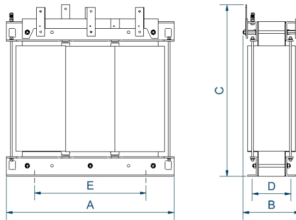
Dimensions (AxBxCxDxE): 1300x550x1350x460x800 mm 17
