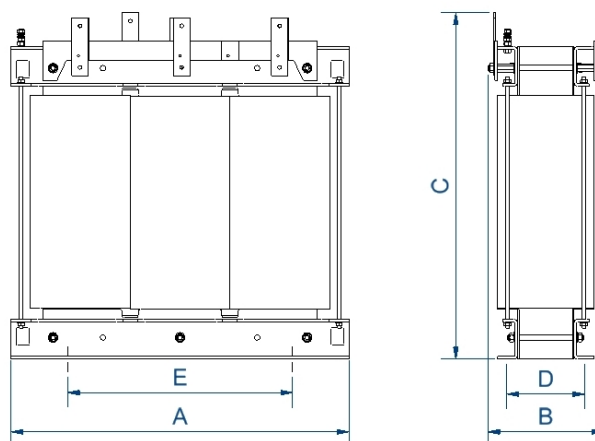
Dimensions (AxBxCxDxE): 1070x550x1220x460x690 mm 17°
