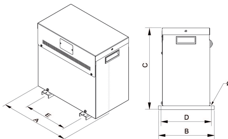
Dimensions (AxBxCxDxE): 528x418x644x375x345 mm 12Ø
