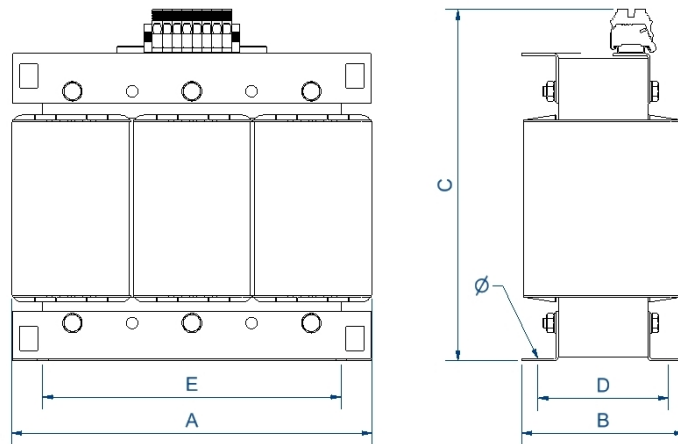
Dimensions (AxBxCxDxE): 180x109x203x91x150 mm 6∅
