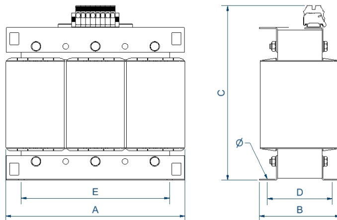
Dimensions (AxBxCxDxE): 480x260x480x154x400 mm 11 \phi
