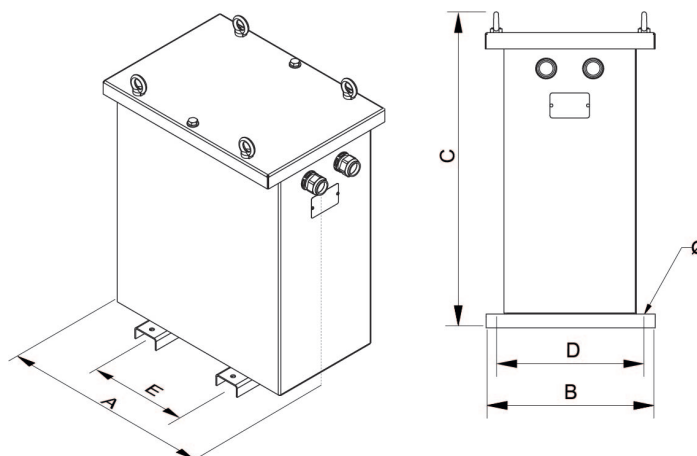
Dimensions (AxBxCxDxE): 510x362x689x320x250 mm 11Ø
