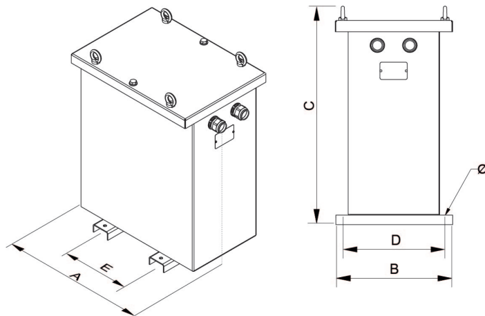
Dimensions (AxBxCxDxE): 694x413x764x370x350 mm 110
