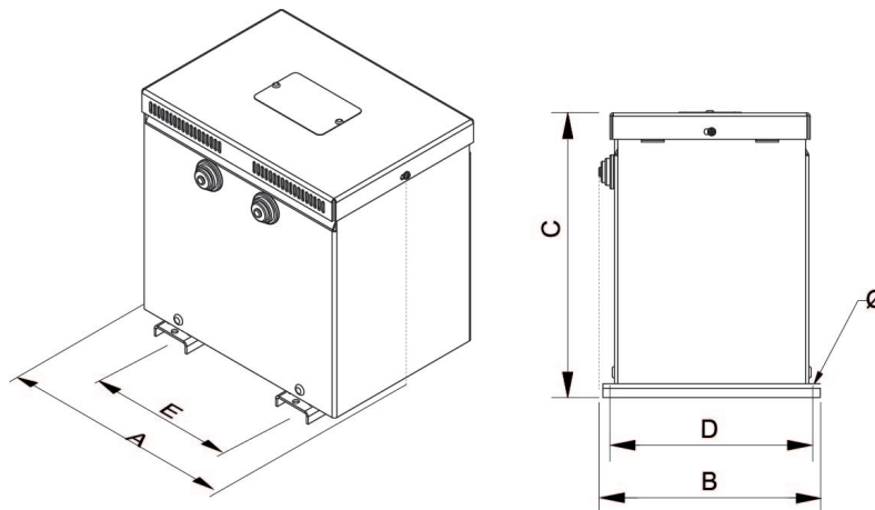
Dimensions (AxBxCxDxE): 194x175x220x165x100 mm 6Ø
