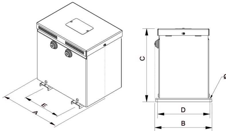
Dimensions (AxBxCxDxE): 380x260x384x245x250 mm 6Ø
