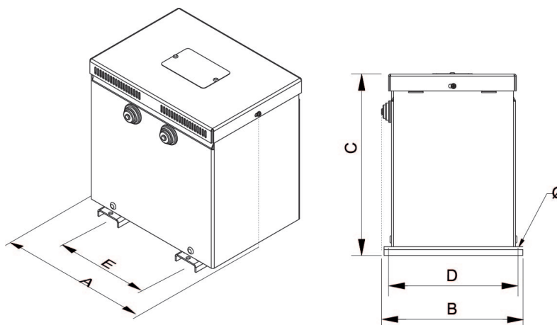
Dimensions (AxBxCxDxE): 817x560x975x500x415 mm 12Ø
