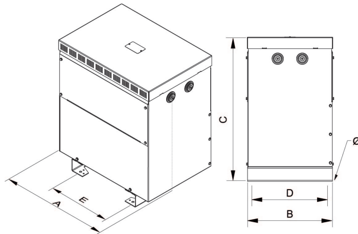
Dimensions (AxBxCxDxE): 480x340x500x300x300 mm 12Ø
