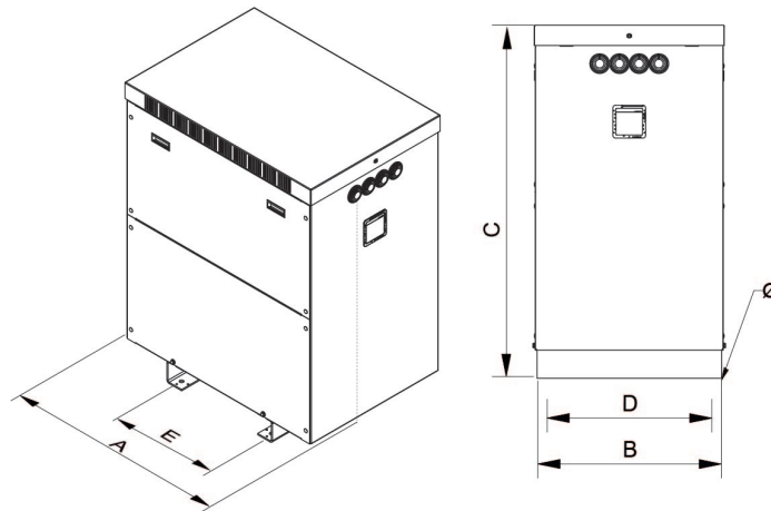
Dimensions (AxBxCxDxE): 480x340x500x300x300 mm 12Ø
