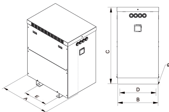
Dimensions (AxBxCxDxE): 990x670x1250x582x470 mm 18Ø
