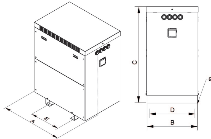
Dimensions (AxBxCxDxE): 597x415x710x375x345 mm 12Ø
