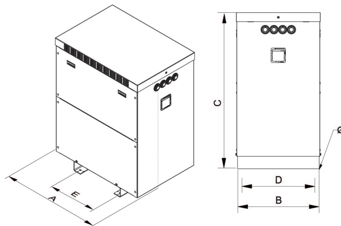
Dimensions (AxBxCxDxE): 1200x770x1555x672x690 mm 18Ø
