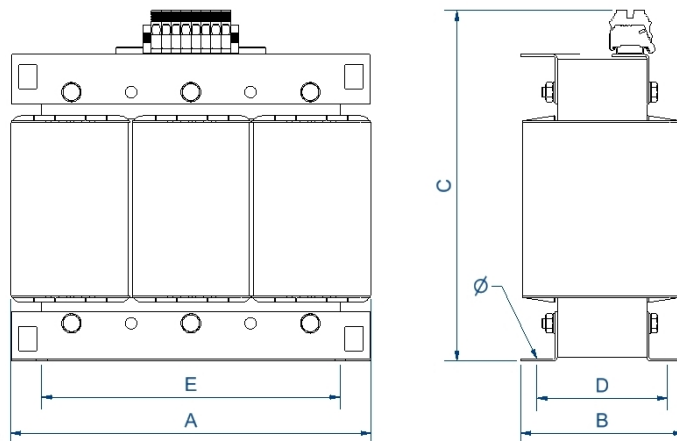
Dimensions (AxBxCxDxE): 360x144x372x122x300 mm 11Ø
