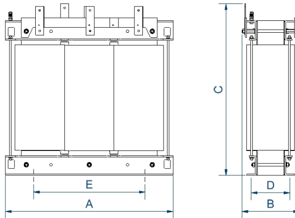
Dimensions (AxBxCxDxE): 714x430x692x189x426 mm 11Ø
