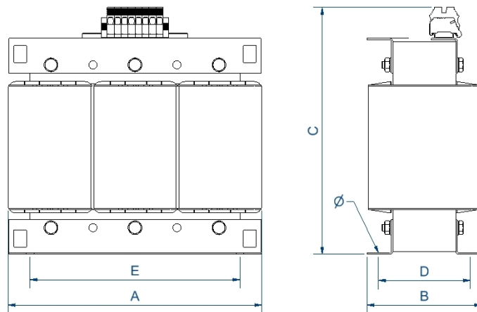
Dimensions (AxBxCxDxE): 360x164x372x142x300 mm 11Ø
