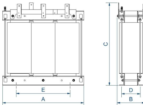
Dimensions (AxBxCxDxE): 1020x550x880x460x470 mm 13Ø
