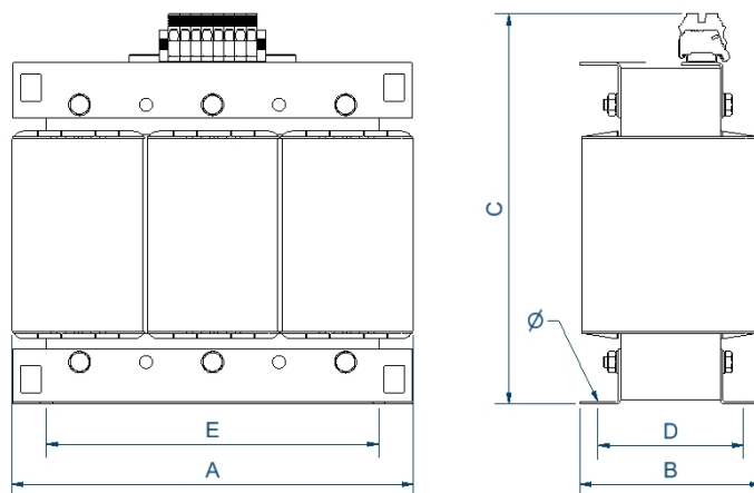
Dimensions (AxBxCxDxE): 420x210x443x182x350 mm 11Ø
