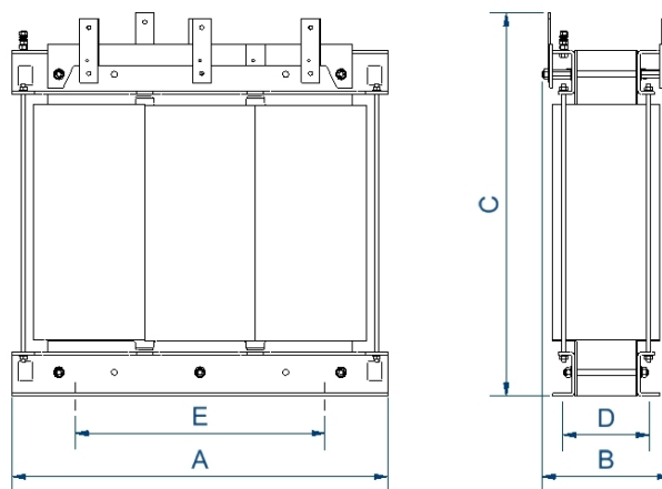
Dimensiones (AxBxCxDxE): 1083x700x1200x600x690 mm 18Ø
