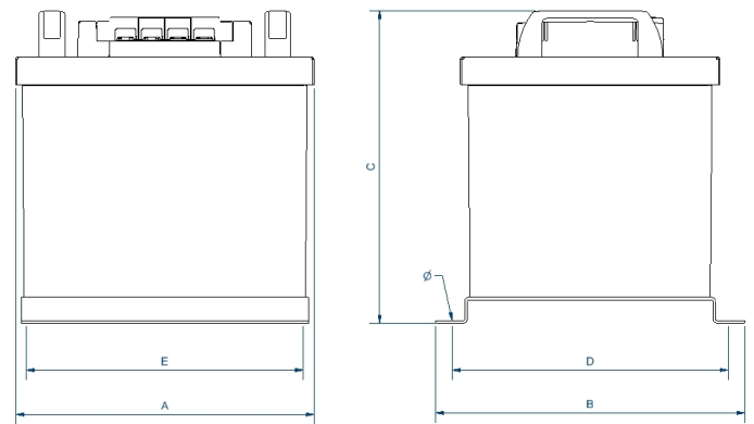
Dimensions (AxBxCxDxE): 233x241x314x219x175 mm 7∅
