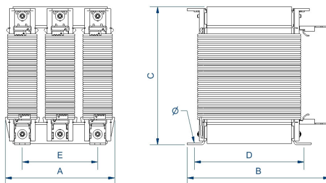
Dimensions (AxBxCxDxE): 150x110x184,5x49x100 mm 6Ø
