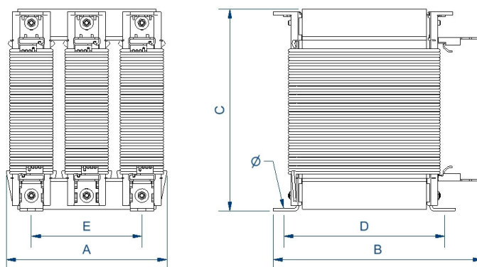
Dimensions (AxBxCxDxE): 150x120x185x59x100 mm 6Ø
