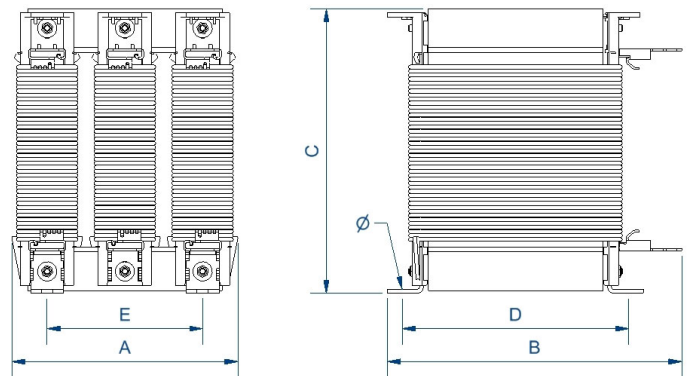
Dimensions (AxBxCxDxE): 150x120x185x59x100 mm 6Ø
