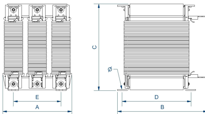
Dimensions (AxBxCxDxE): 370x350x600x274x140 mm 11Ø
