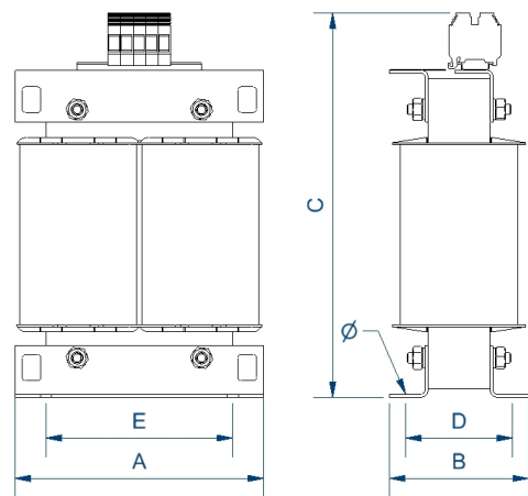
Dimensions (AxBxCxDxE): 200x164x303x155x154 mm 9Ø
