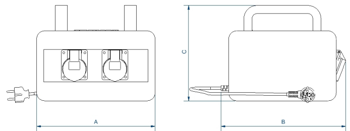
Dimensions (AxBxCxDxE): 215x210x180 mm
