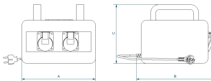
Dimensions (AxBxCxDxE): 245x300x235 mm
