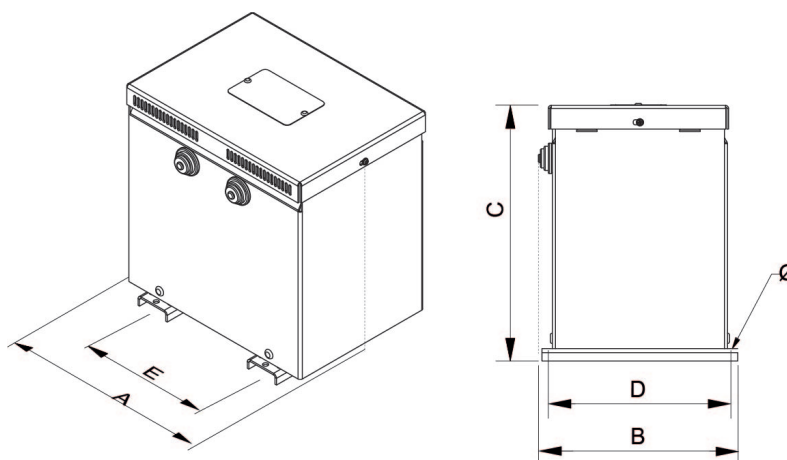
Dimensions (AxBxCxDxE): 194x175x220x165x100 mm 6∅
