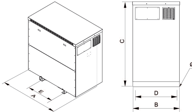
Dimensions (AxBxCxDxE): 1820x1000x1800x900x790 mm 20Ø
