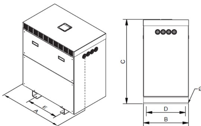
Dimensions (AxBxCxDxE): 1195x760x1560x672x690 mm 18Ø
