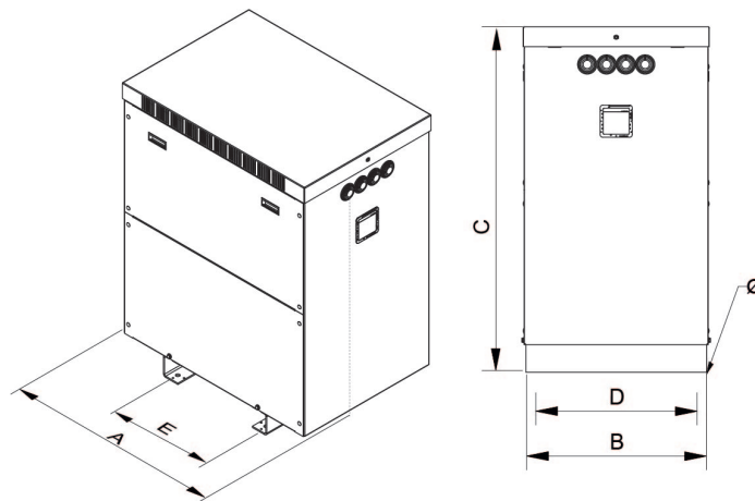
Dimensions (AxBxCxDxE): 1820x1000x1800x900x790 mm 20φ
