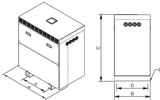
Dimensions (AxBxCxDxE): 985x675x1310x475x470 mm 18Ø
