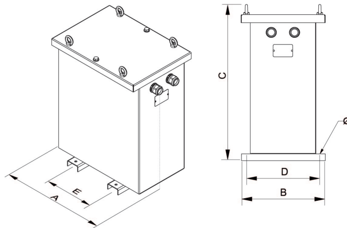
Dimensions (AxBxCxDxE): 890x625x1148x500x426 mm 12Ø
