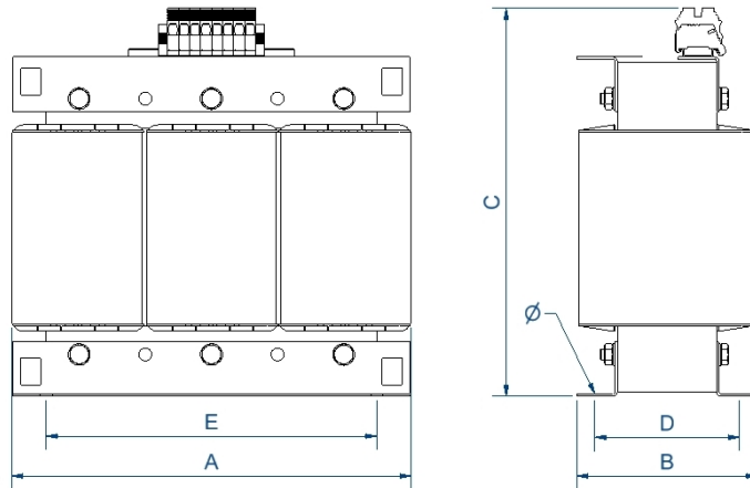
Dimensions (AxBxCxDxE): 150x94x178x66x125 mm 6
