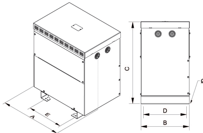
Dimensions (AxBxCxDxE): 458x340x500x300x300 mm 12Ø
