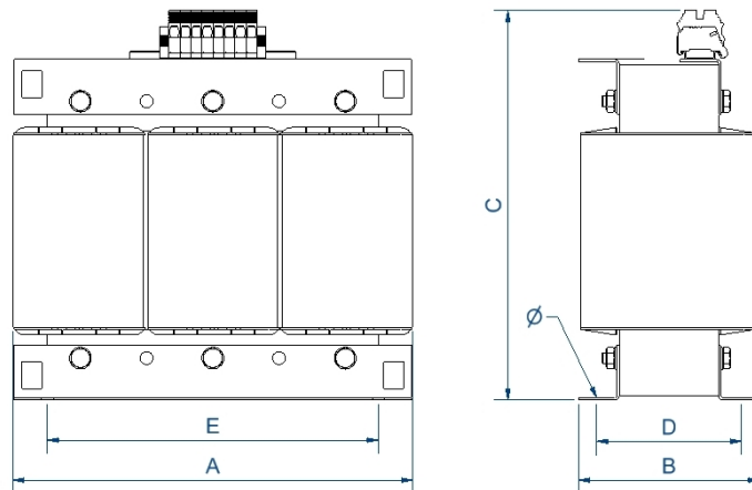
Dimensions (AxBxCxDxE): 300x154x303x145x250 mm 9Ø
