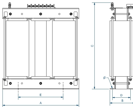
Dimensions (AxBxCxDxE): 740x290x580x170x426 mm 13Ø
