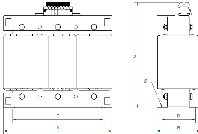
Dimensions (AxBxCxDxE): 400x144x353x122x300 mm 11Ø
