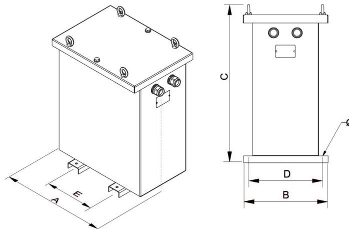
Dimensions (AxBxCxDxE): 970x625x1150x500x426 mm 12Ø
