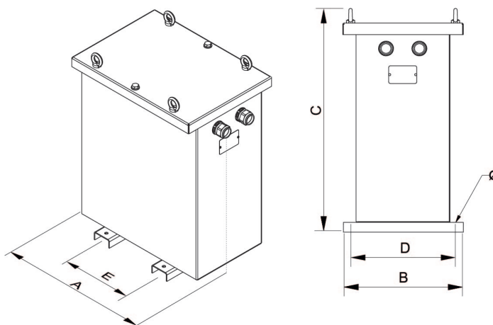
Dimensions (AxBxCxDxE): 510x362x689x320x250 mm 11Ø
