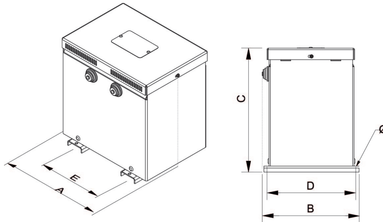
Dimensions (AxBxCxDxE): 240x190x250x180x150 mm 6Ø
