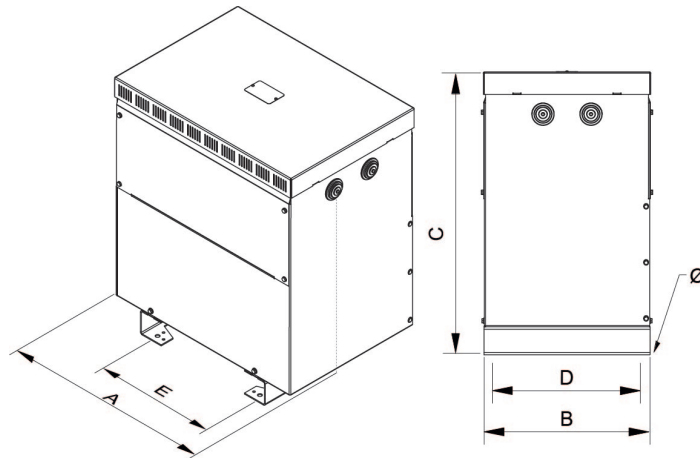
Dimensions (AxBxCxDxE): 597x415x710x375x350 mm 12Ø
