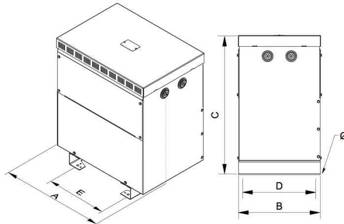
Dimensions (AxBxCxDxE): 597x415x710x375x350 mm 12
