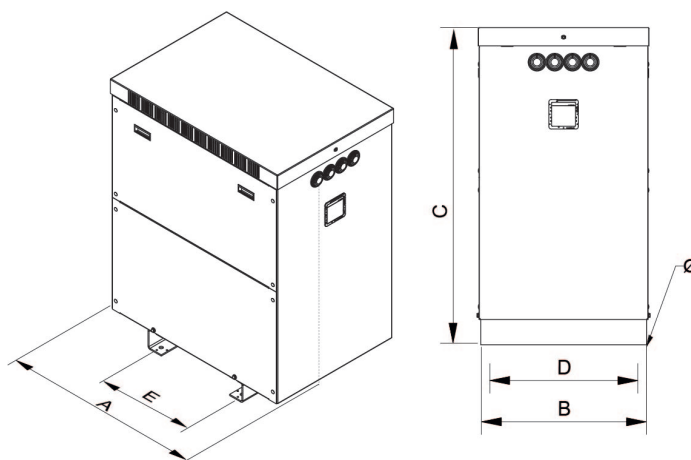
Dimensions (AxBxCxDxE): 990x685x1255x582x470 mm 18Ø
