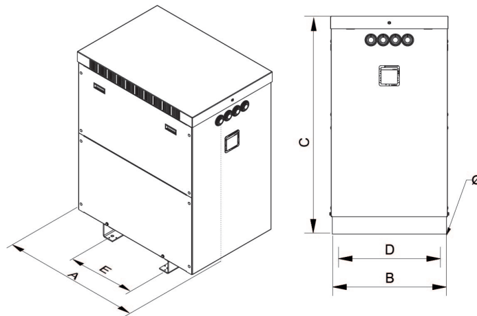
Dimensions (AxBxCxDxE): 1215x775x1555x672x690 mm 18Ø
