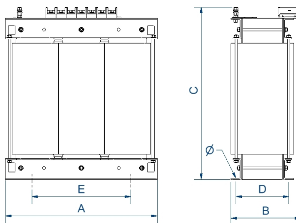
Dimensions (AxBxCxDxE): 714x420x637x209x426 mm 11Ø
