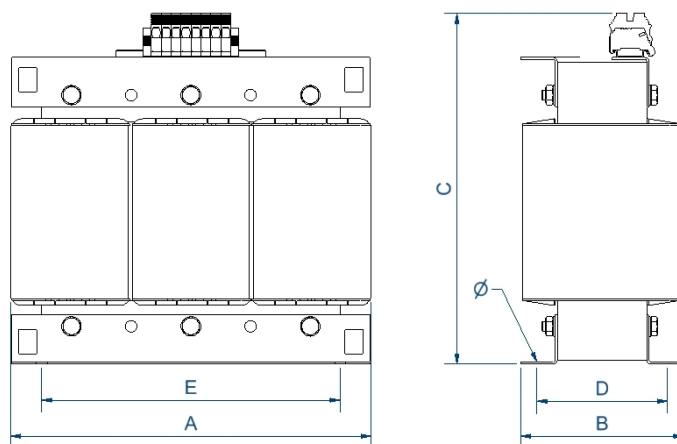
Dimensions (AxBxCxDxE): 480x194x465x115x400 mm 11Ø
